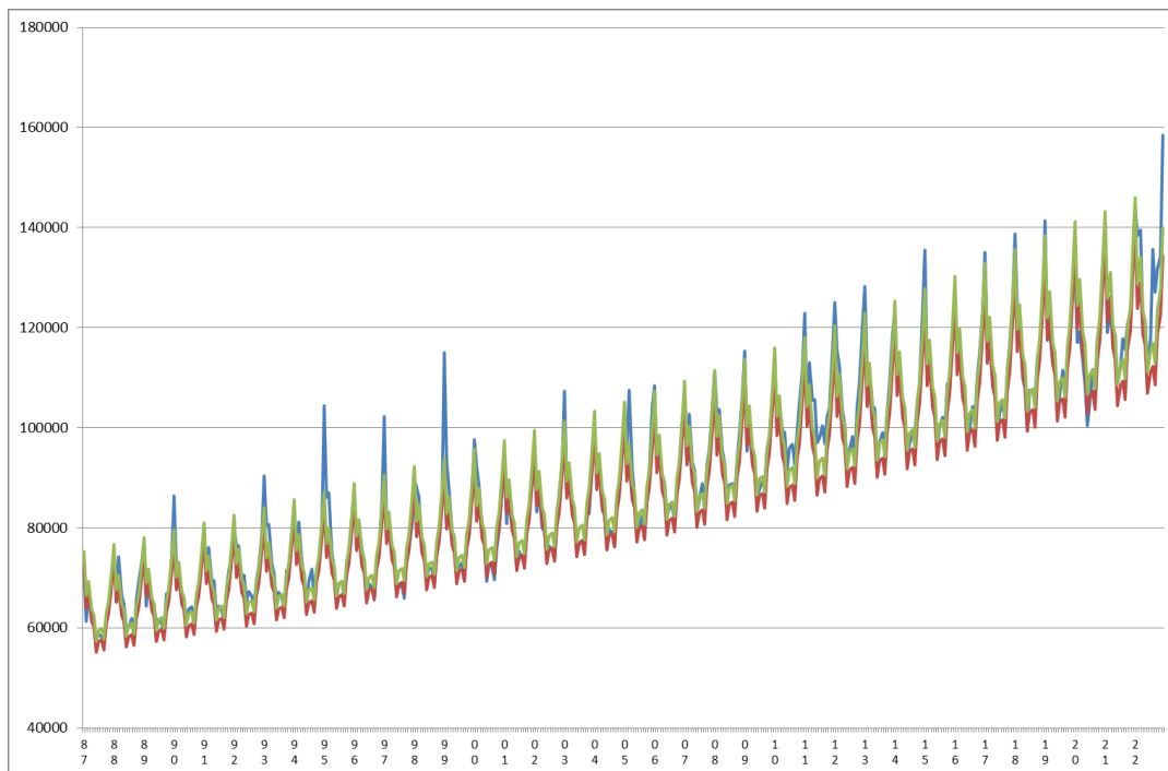
Figure 1: Observations of the estimated baseline and threshold since 1987 until December 2022 in Japan
