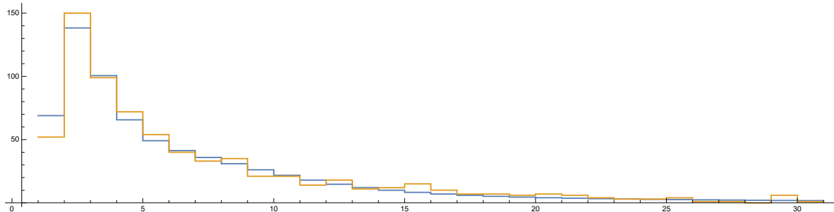
FIGURE 2. Comparison of the vaccination model described above with [1, Figure 2], 1 \leq k \leq 30
