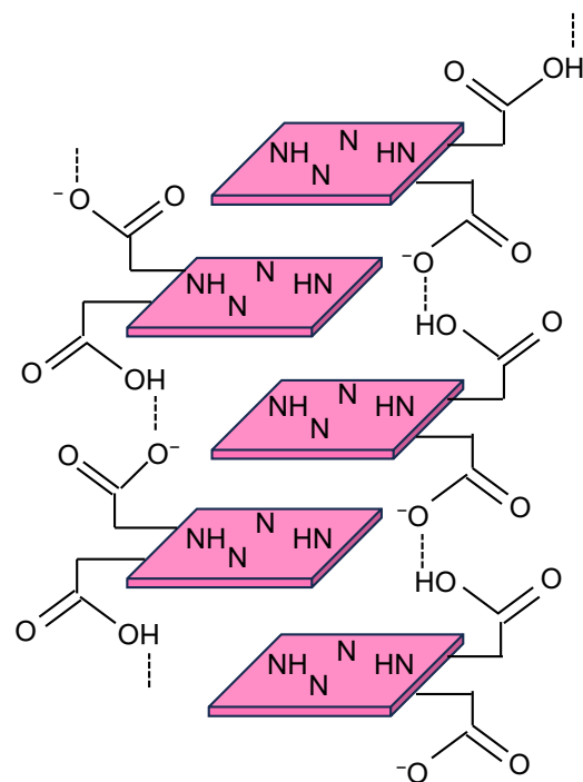
J-aggregate
